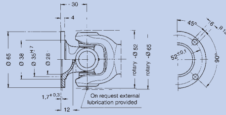
On both sides larger flange end number: 0.105.XX1
