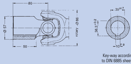
On both sides connecting hub without key-way end number: 0.109.XX2 with key-way end number: 0.109.XX3
