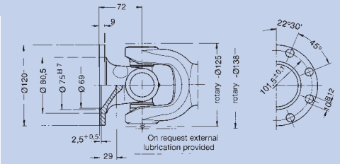
Flange for larger angle of deflection end number: 0.113.XX5
