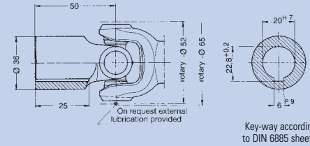
On both sides connecting hub without key-way end number: 0.105.XX2 with key-way end number: 0.105.XX3
