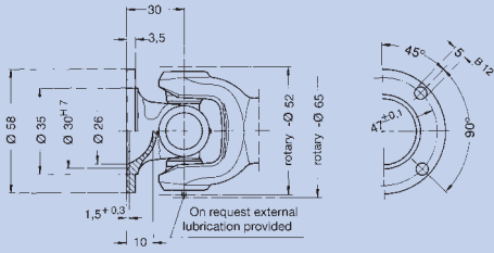
On both sides standard flange end number: 0.105.XX0
